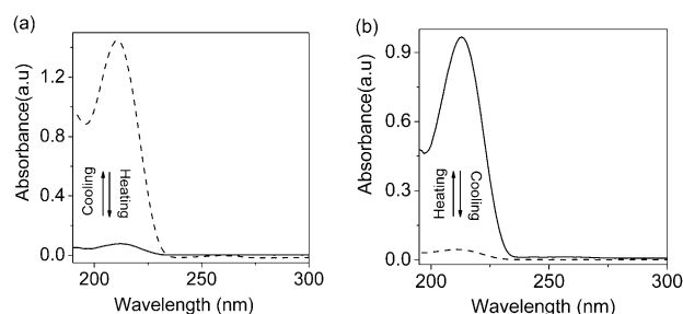
Figure 2. UV-vis spectra of [\text{PEG}_{1000}(\text{mim})_2][\text{NTf}_2]_2 before and after phase transfer between \text{H}_2\text{O} and EA upon heating (solid, 50^\circ\text{C} ) and cooling (dotted, 20^\circ\text{C} ) as shown in Figure 1. The IL was originally dispersed in water (15 wt% IL) at 20^\circ\text{C} . a) \text{H}_2\text{O} . b) EA.
